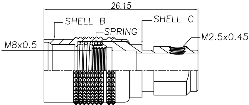
SHELL B + SHELL C + SPRING
