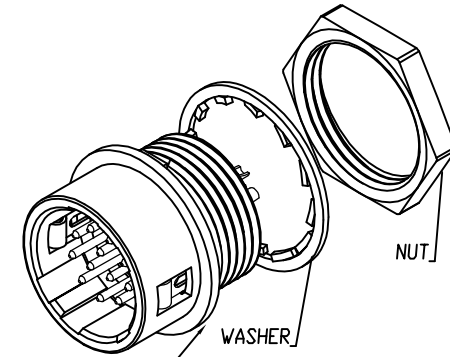
HOUSING+CONTACT+SPRING+SHELL
