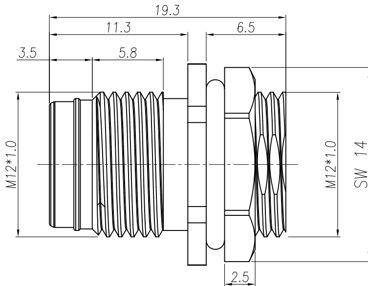
SHELL+O-RING +NUT
